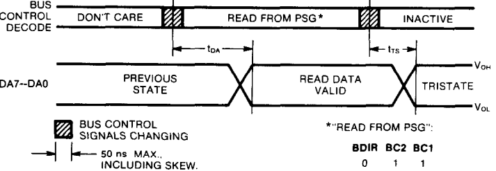
Fig. 40 READ DATA TIMING
